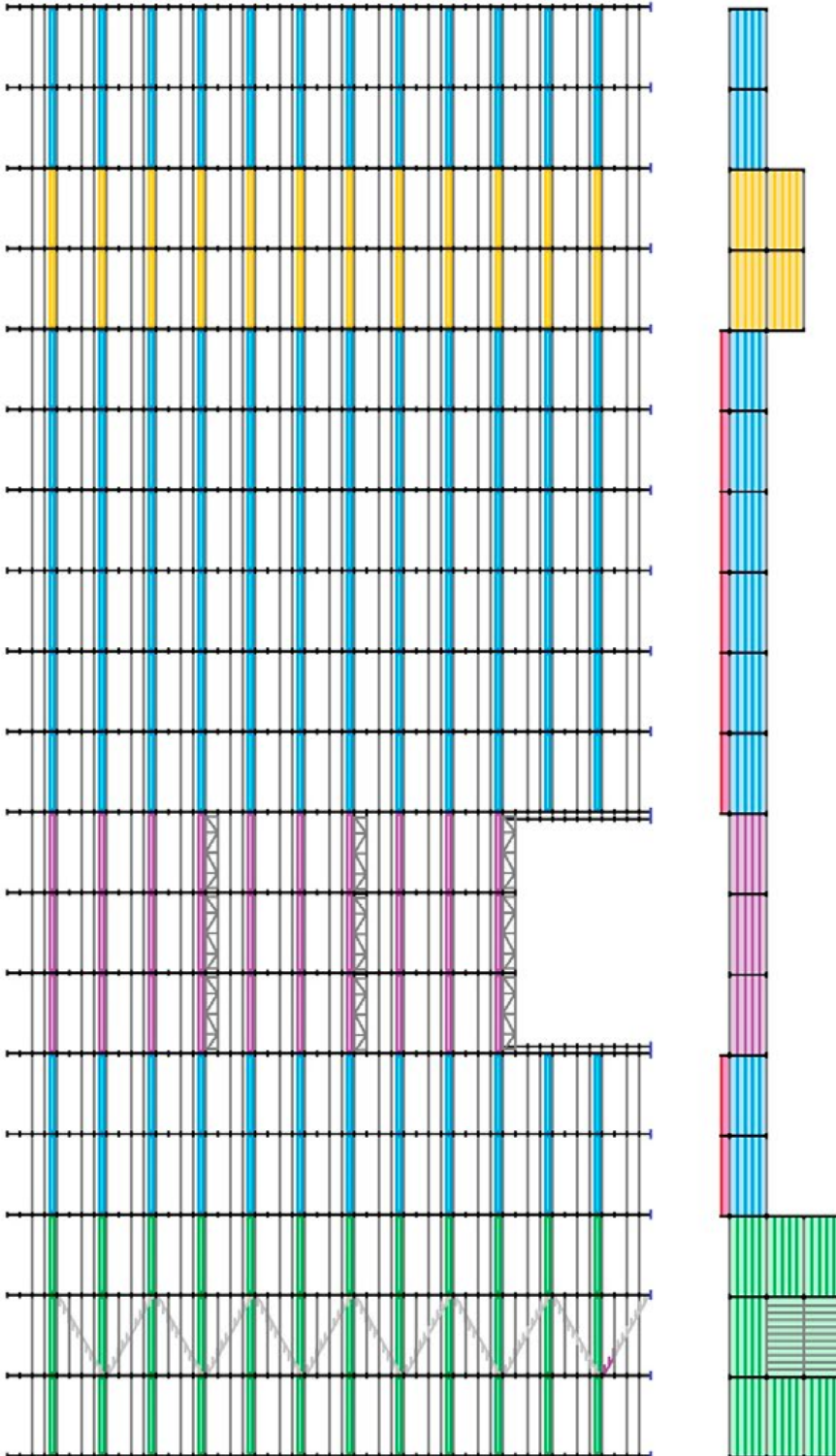
Figure E5. Example scaffold design – design loading
