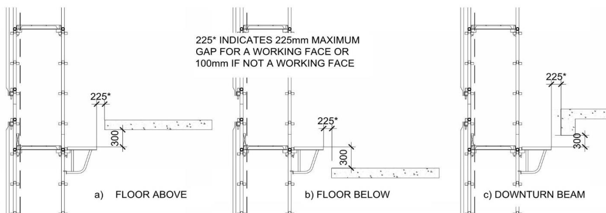
Figure 8 Allowable gaps
