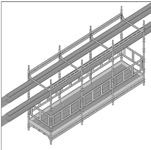
Figure 13 Hung scaffold 4
