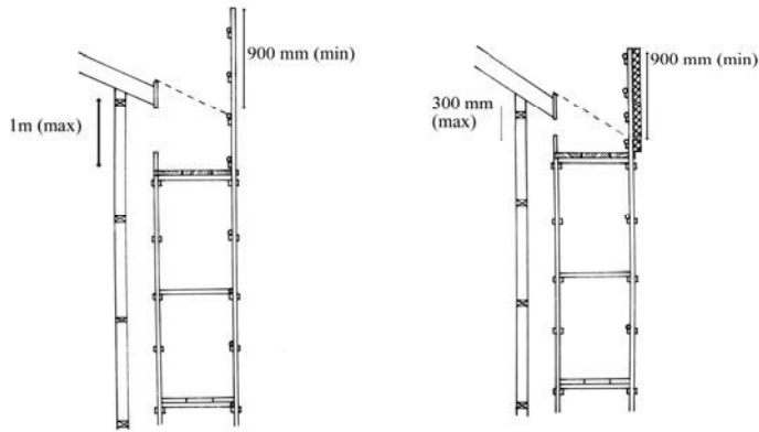
Figure 7a Fall arresting platform \leq 26^\circ
