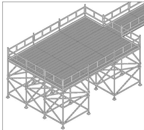
Figure 11 Birdcage scaffold 3
